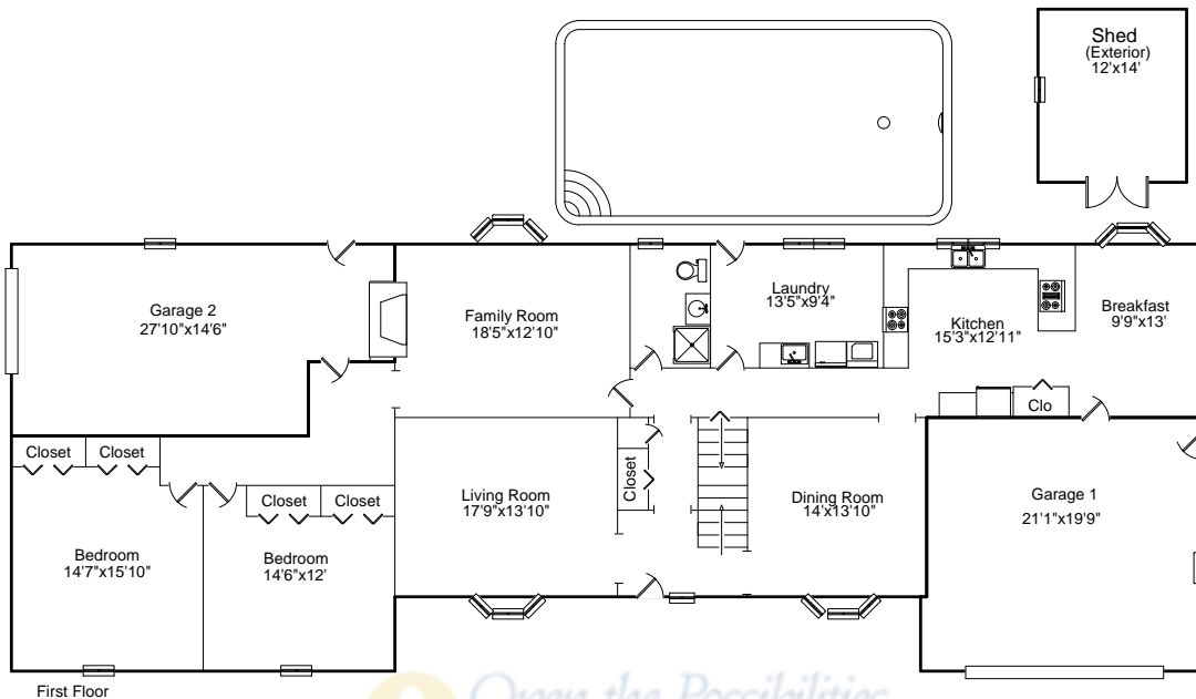
First Floor
