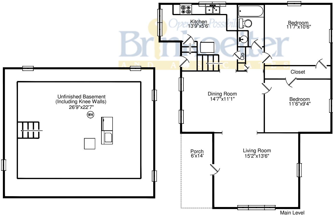
Main Level
